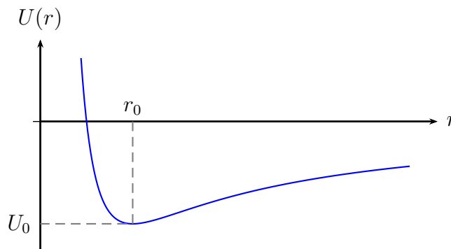
Figure 1: Potential energy U(r) as a function of distance r .
