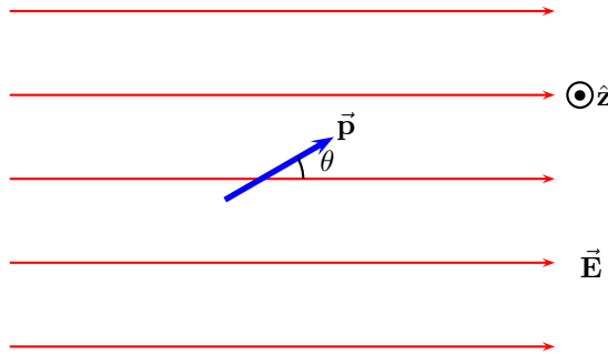
Figure 25.5: Electric dipole in a uniform electric field.
