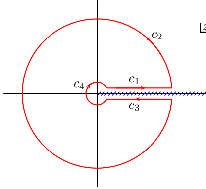
Figure 3.4: Contour c = c_1 + c_2 + c_3 + c_4 . The radii of the contours c_2 and c_4 are R and \epsilon , respectively, and contours c_1 and c_3 are \delta away from the real line. We assume limits \epsilon \rightarrow 0 , R \rightarrow \infty , and \delta \rightarrow 0 .
